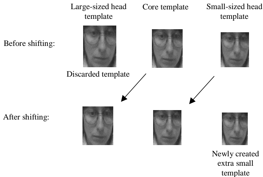
Figure 3-3 Shifting Process
