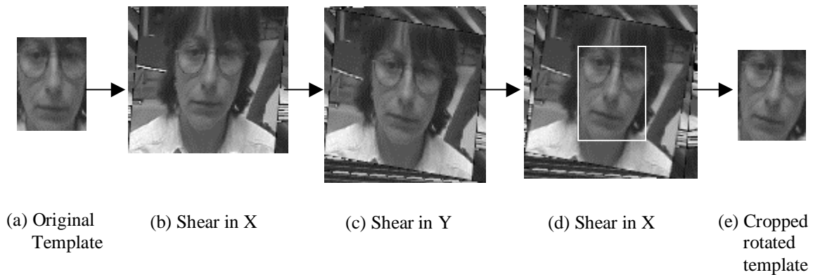
Figure 4-4 Rotation Algorithm
