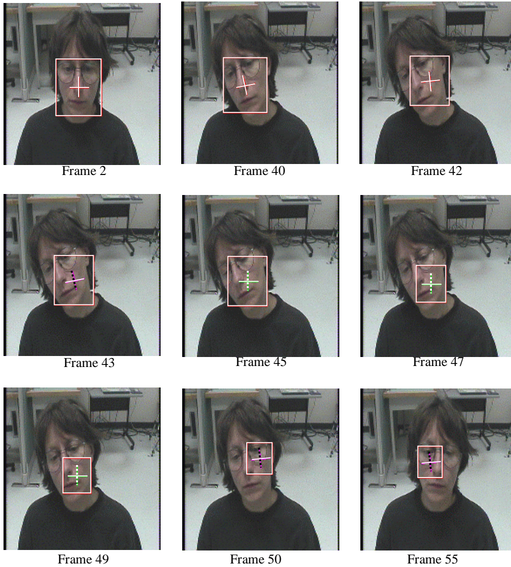
Figure 5-5 Tracking Failure
