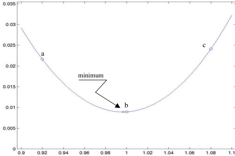
Figure 3-2 Interpolation Process
