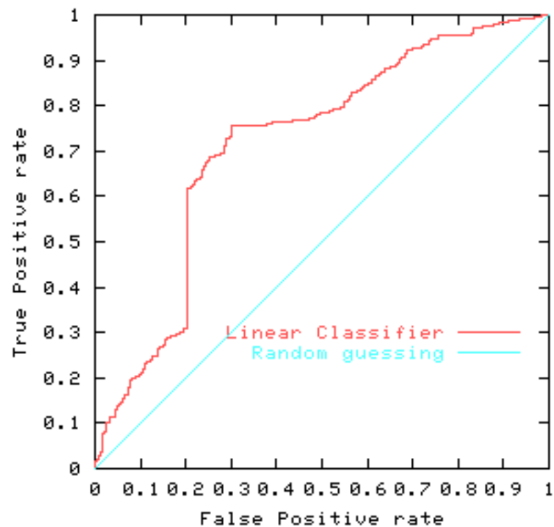
Thyroid anomaly detection
