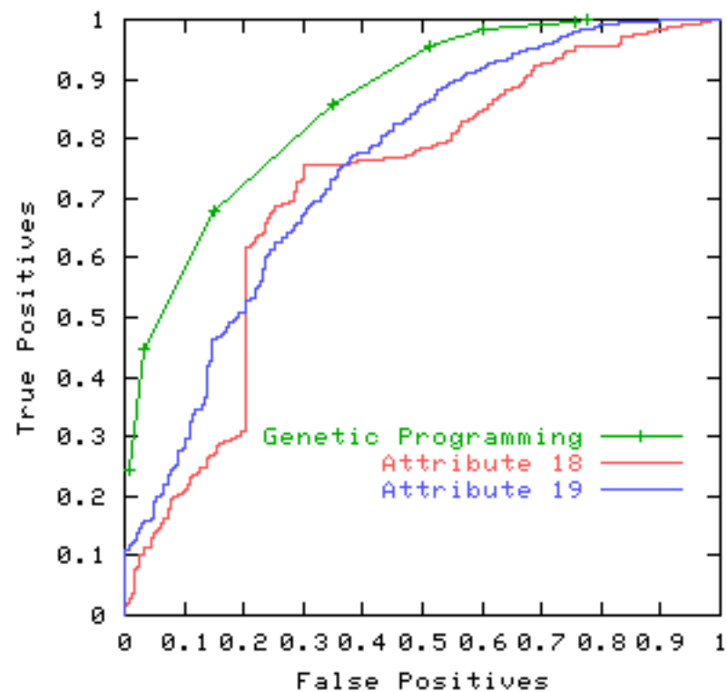
Thyroid Evolved Classifier
