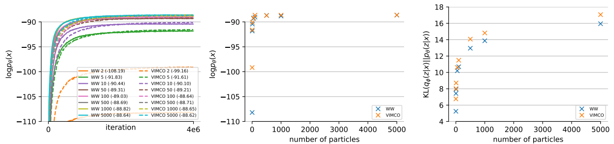
Figure 13: Training of sigmoid belief nets. (Left) Training curves: WW learns faster than VIMCO but results in equal or slightly worse end test log likelihood. (Middle) Log evidence values at the end of training: VIMCO is slightly better than WW in low-particle regimes but virtually the same in high-particle regimes. (Right) KL divergence at the end of training: WW results in much lower KL divergence than VIMCO.
