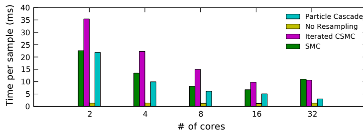
Figure 4: Average time to draw a single complete particle on a variety of machine architectures. Queuing rather than blocking at each observation improves performance, and appears to improve relative performance even more as the available compute resources increase. Note that we see only average time per sample, here; this is not a measure of statistical efficiency. The high speed of the non-resampling algorithm is not sufficient to make it competitive with the other approaches.
