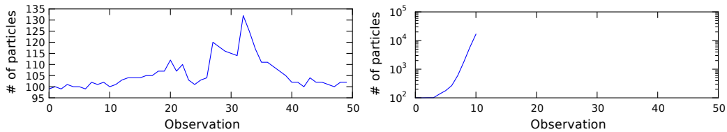
Figure 1: Number of particles K_n at each of n = 0, \dots, 49 for a one-dimensional linear Gaussian model, initialized with 100 particles. (left) When the order of the particles arriving at each n is subject to a random permutation, then the number of particles is reasonably stable, staying at or near 100. (right) When the order of the particles arriving at each n is completely deterministic, then the total number of particles quickly explodes, in this case exceeding 15000 by n = 11 .
