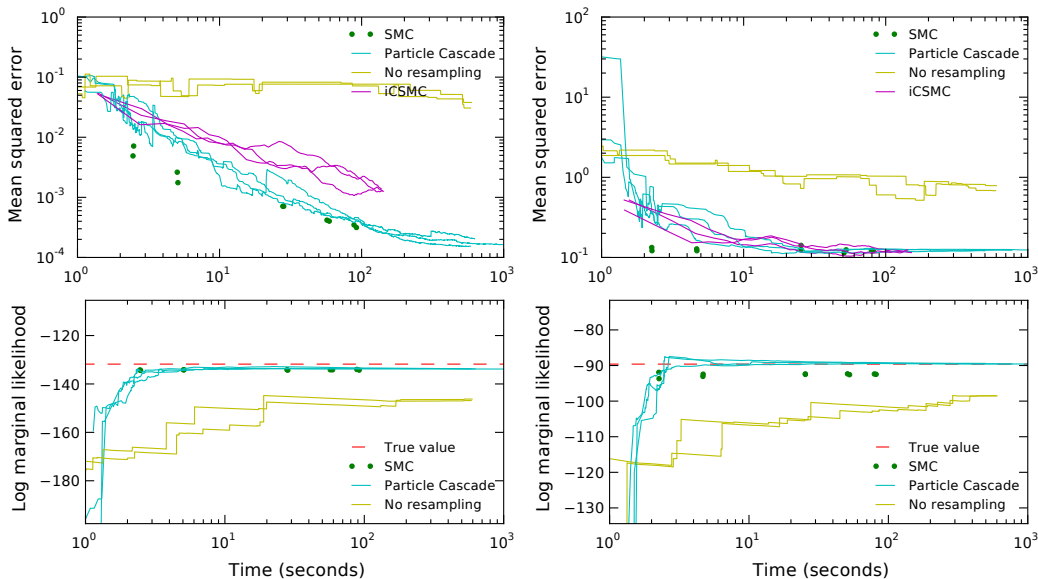
Figure 3: (top) Comparative convergence rates between SMC alternatives including our new algorithm, and (bottom) estimation of marginal likelihood, by time. Results are shown for (left) the hidden Markov model, and (right) the linear Gaussian state space model.
