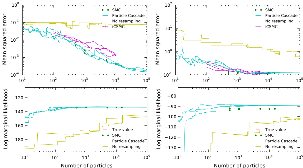
Figure 2: All results are reported over multiple independent replications, shown here as independent lines. (top) Convergence of estimates to ground truth vs. number of particles, shown as (left) MSE of marginal probabilities of being in each state for every observation n in the HMM, and (right) MSE of the latent expected position in the linear Gaussian state space model. (bottom) Convergence of marginal likelihood estimates to the ground truth value (marked by a red dashed line), for (left) the HMM, and (right) the linear Gaussian model.
