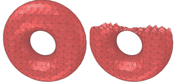
Figure 4: Tetrahedral mesh of a torus (8.5K elements). Using the principal curvatures increases the level of resolution in the inner ring.
