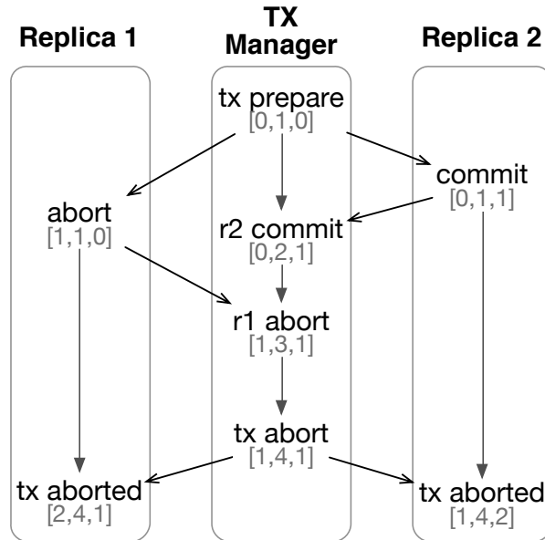
Fig. 1. Time-space diagram illustrating an execution of the two-phase commit protocol [9] with one transaction manager and two replicas. The vertical lines represent the host ordering, and the diagonal lines represent the interaction ordering. Each event has an associated vector timestamp. For conciseness, this time-space diagram does not explicitly include message send and receive events.
