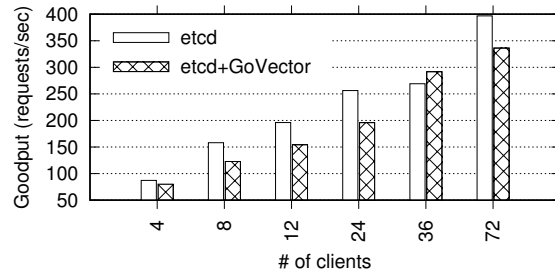
Fig. 11. Goodput of uninstrumented and instrumented etcd Raft.
