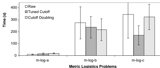
Figure 8: Solution times for two types of random restarts. Tuned cutoff uses raw experimental data to select a constant cutoff. Cutoff doubling starts with a cutoff of one second and doubles it on each run.
