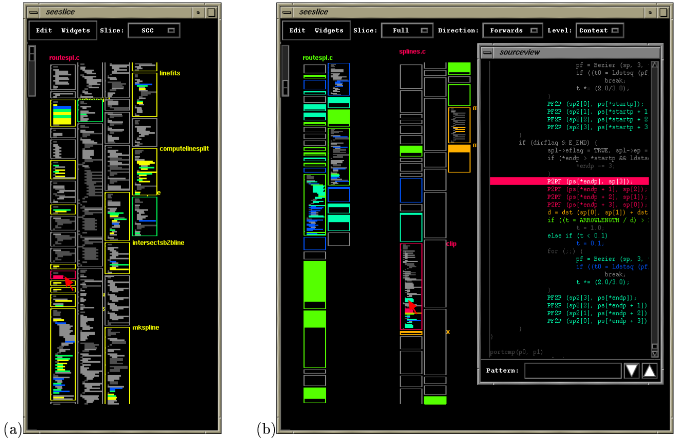
Figure 11: Program Slices . Two views from the SeeSlice system. Panel (a) shows a slice in one file. Panel (b) displays a forward slice spanning two files (the slice point is red). Some procedures have been “closed” to hide their line representations.
