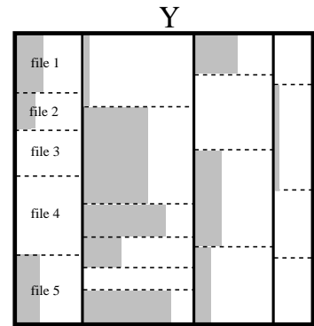
Figure 5: Hierarchical representation . Subsystem and directory statistics (a), a fill statistic for directories (b), and a zoomed view on subsystem Y showing file level statistics (c).
