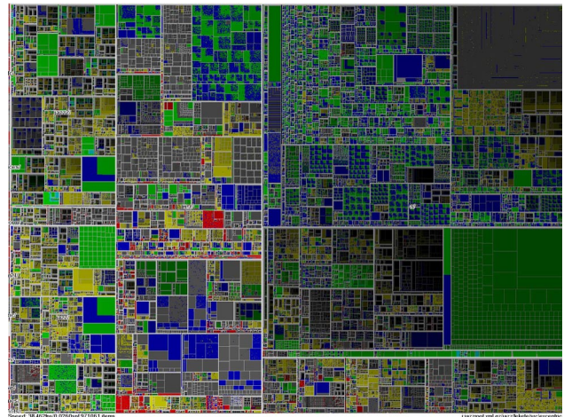
Figure 1: This treemap gives an overview of the 970,000 files of a large file system on a 1600x1200 display. The size of each rectangle is determined by the file's size; color represents file type. Deeply nested directories appear darker.
