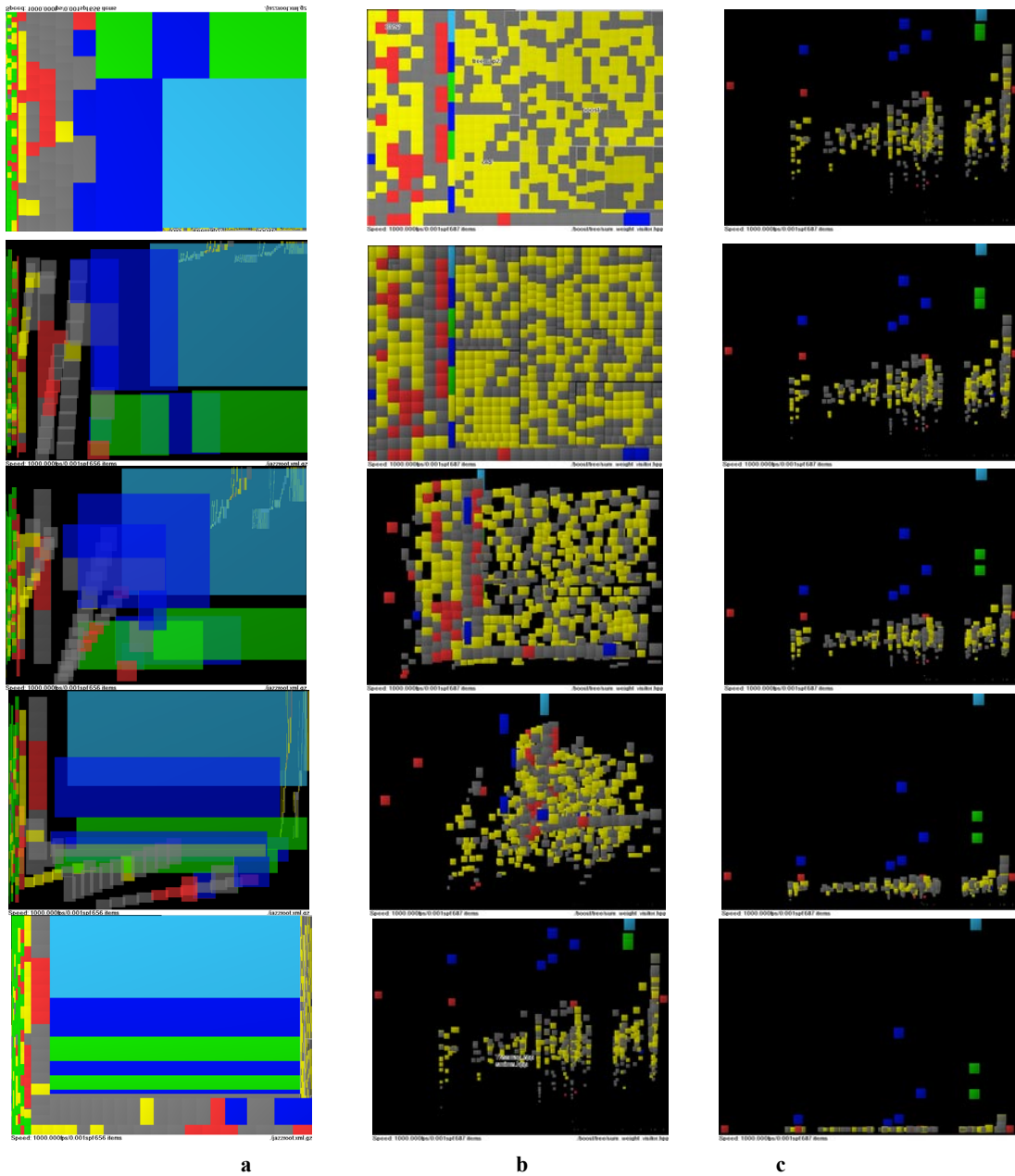
Figure 5: Animation of visualizations using linear interpolation: a) interpolation between two different treemap layouts - squarified to slice and dice, b) interpolation between a treemap and a scatter plot, c) interpolation corresponding to a change of attribute for the Y axis on a scatter plot.
