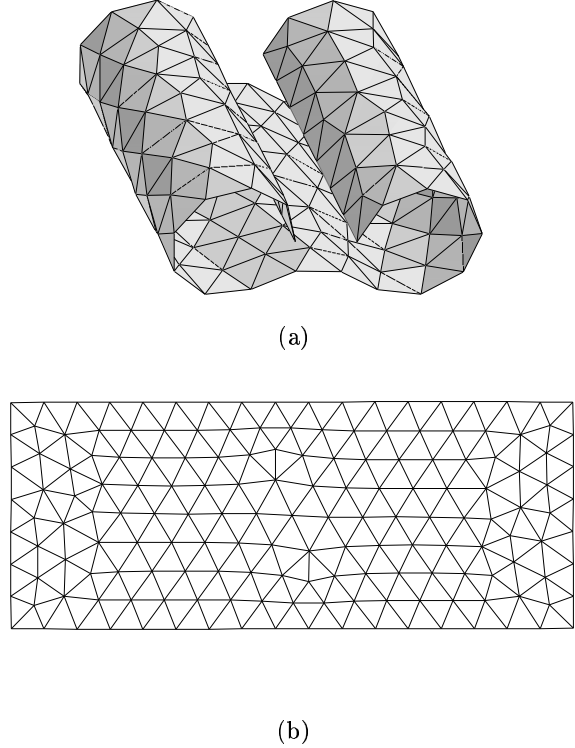
Figure 9. Flat triangulation of nearly developable surface. (a) Original model. (b) Flat triangulation.
