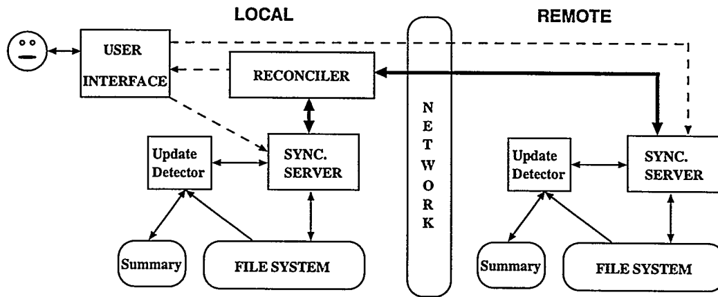
Figure 2: Internals of our synchronizer
