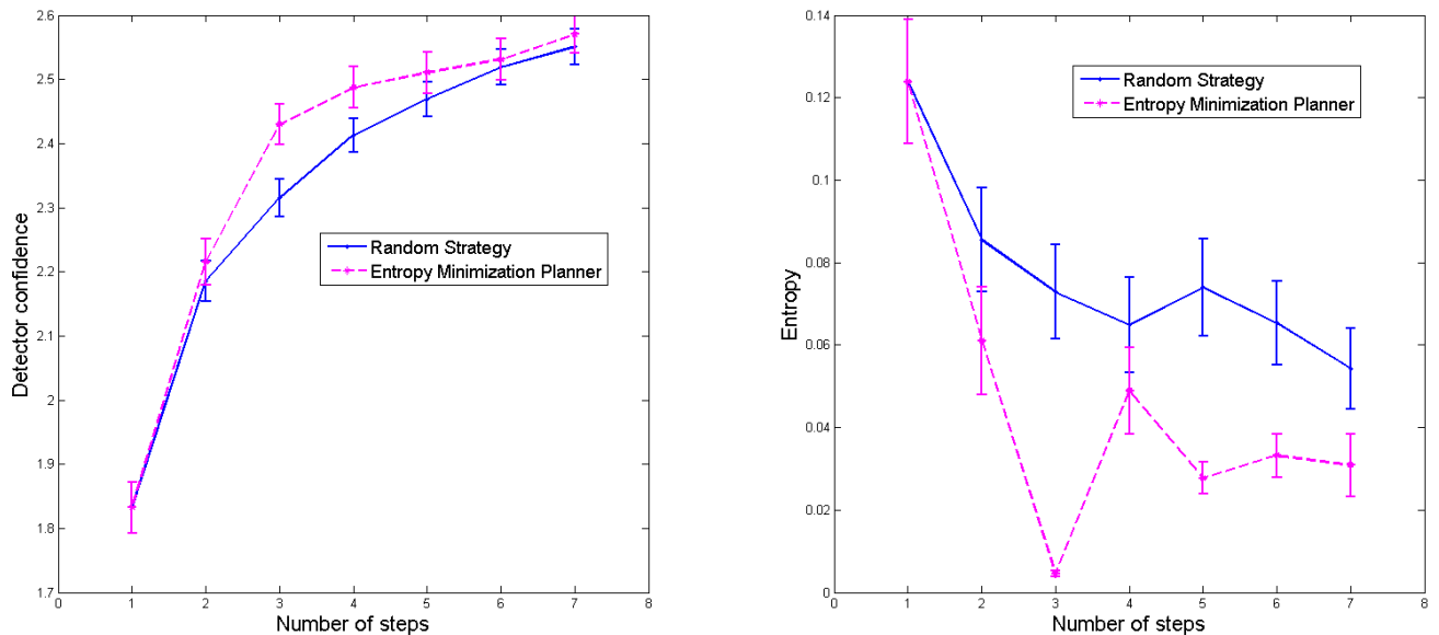
Fig. 5. A comparison of detection results between a system using entropy minimization planning and a system which uses a random planning strategy. The graph on the left shows the sum of positive detector responses for true positives plus the sum of negative responses for true negatives, an approximation to precision and recall. The graph on the right shows the entropy of the marginal p(o = x) , the detector’s belief in the true category label x . All results are averages over 160 random selections of an object instance and starting viewpoint.
