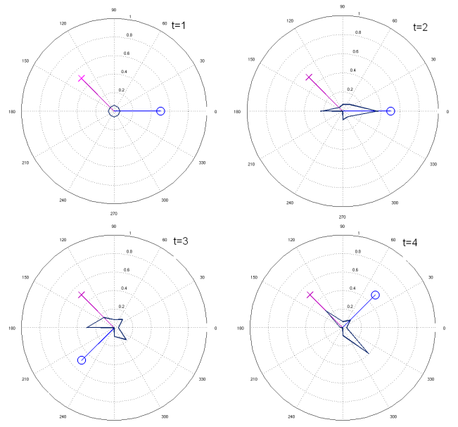
Fig. 4. The posterior, p(o = x, \theta | f_1, \dots, f_t) is displayed as the radial coordinate and is shown evolving over a number of views observed for the category label “car”. The magenta “x” shows the pose of the object and the blue circle shows the robot’s pose at each time step.
