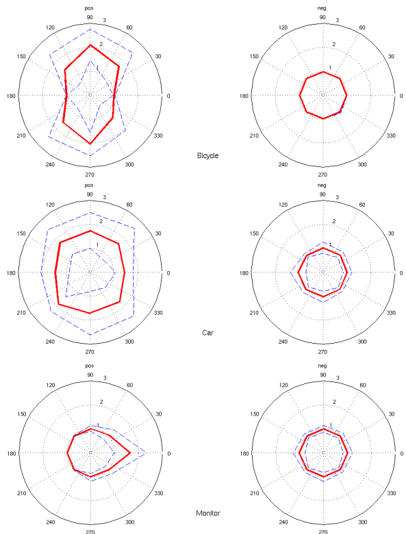
Fig. 2. Example viewpoint detection functions of the deformable parts model detector for classes: (top) bicycle, (middle) car, and (bottom) monitor. The radial coordinate represents the detector response to positive(left) and negative(right) samples. The solid red line is the expected value and dotted blue lines depict the uncertainty in the response.
