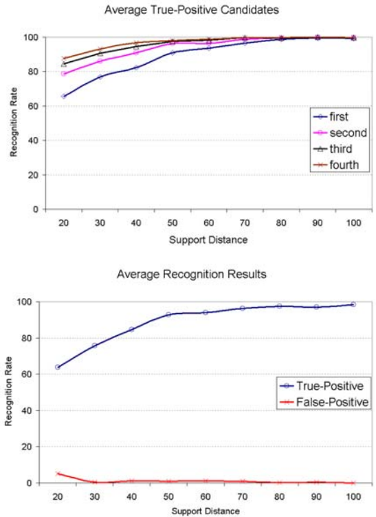
Fig. 7 Average of recognition results for noisy test models. Top: Positive candidate selection. Bottom: True-positive recognition rate
