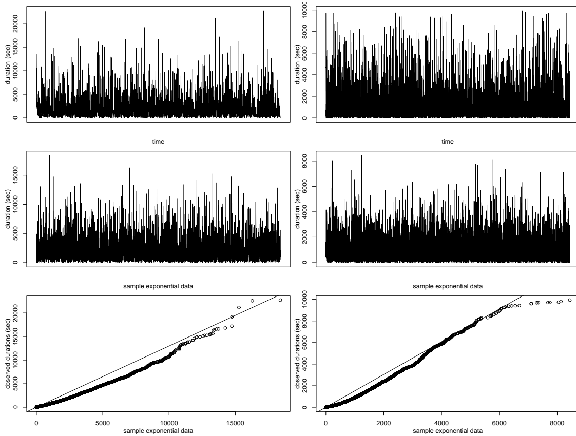
Figure 9: Fitting an exponential distribution to user duration data
