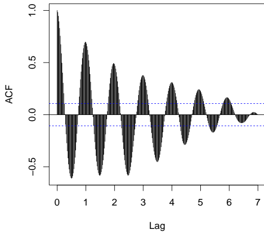
(c) ACF of Figure 3(a)
