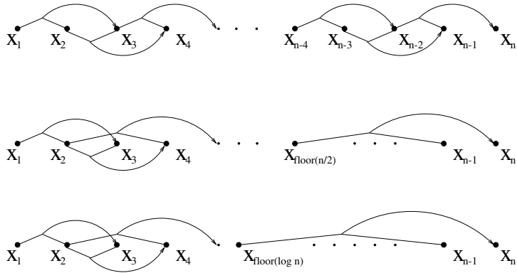
Fig. 6. These three diagrams illustrate our ternary chain formulas. The top panel shows F_{3chain,i-2} which has local links in the form of x_{i-2} \wedge x_{i-1} \rightarrow x_i only. The middle panel gives F_{3chain, \lfloor \frac{i}{2} \rfloor} which has longer links of the form x_{\lfloor \frac{i}{2} \rfloor} \wedge x_{i-1} \rightarrow x_i . The bottom panel shows F_{3chain, \lfloor \log i \rfloor} with even longer links of the form of x_{\lfloor \log i \rfloor} \wedge x_{i-1} \rightarrow x_i
