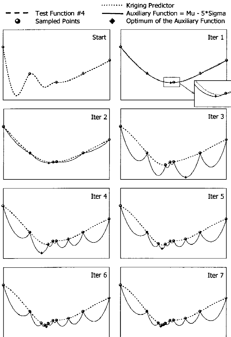
Figure 13. Selected iterations of Method 3 on a simple one-dimensional test function. In each iteration, we fit a kriging surface to the data, find the point that minimizes the predictor minus \kappa standard errors, and then evaluate the function at this point.
