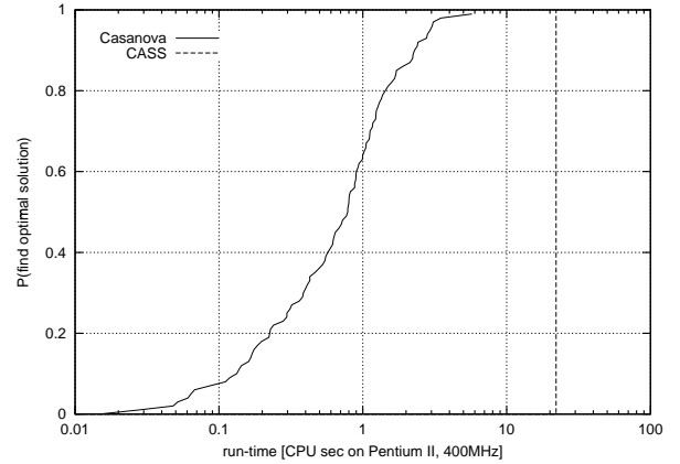
Figure 4: Regular bids, typical instance from test set UNI-3-100-100: Empirical RTDs for finding the optimal solution using Casanova vs. CASS, based on 100 runs for Casanova, one deterministic run for CASS.
