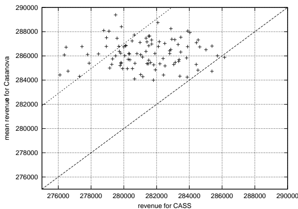
Figure 1: Regular bids, test set UNI-3-200-10000: Correlation of (mean) revenue obtained by CASS and Casanova within a fixed cutoff time of 60 CPU sec. The two lines show ratio of 1 and 1.025 when comparing the revenue obtained by Casanova to that of CASS.
