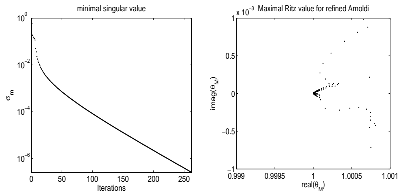
FIG. 4.2. Eigenvalues and singular values for the edu matrix, with c = 0.99 and k = 4 . (Most of the Ritz values corresponding to the first 21 iterations were not within the bounds of the graph and are not shown.)
