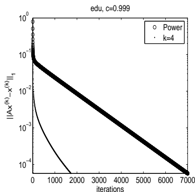
FIG. 4.1. Convergence behavior for the 2,024,716 \times 2,024,716 edu matrix, with c = 0.999 .
