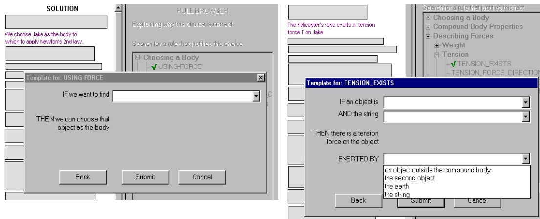
Figure 8: Rule Templates
