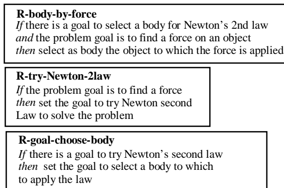
Figure 3: sample rules in the Andes' knowledge base.
