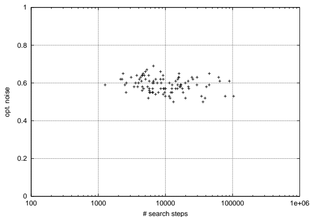
Figure 2: Approx. optimal noise values vs. lsc for Novelty + on test-set flat100-239-100.
