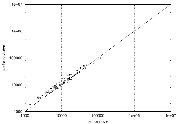
Figure 3: Correlation between lsc for Novelty + with optimal static noise vs. dynamic noise mechanism on test-set flat100-239-100.
