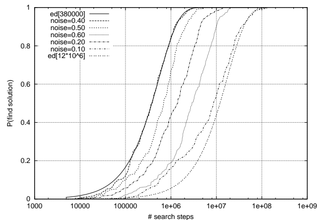
Figure 1: Left : Noise response for Novelty + on easy, medium, and hard instances from test-set flat100-239-100. Right : RTDs for for WalkSAT/SKC on SAT-encoded block world planning instance bw_large.b for approx. optimal, lower and higher noise settings.
