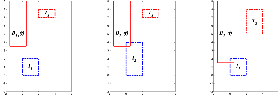
Fig. 3. Backward maximal reach sets B_{I^+}(\mathbf{H}_2, T_i, t) at t = 3.5 for various combinations of initial and target set.
