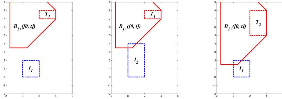
Fig. 4. Backward maximal reach tubes B_{I^+}(\mathbf{H}_2, T_i, [0, t]) at t = 3.5 for various combinations of initial and target set.
