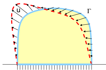
Fig. 2. Illustration of discrete nodal displacements u defined at nodes, e.g., vertices, on the undeformed boundary \Gamma (solid blue line), that result in a deformation of the surface (to dashed red line). Although harder to illustrate, a similar definition exists for the traction vector, p .
