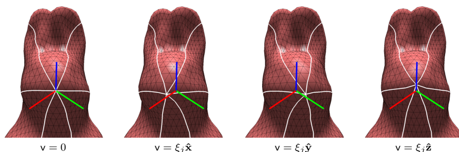
Fig. 3. Illustration of the j^{\text{th}} Green's function block column, \xi_j = \Xi_{:j} , representing the model's response due to the three XYZ components of the j^{\text{th}} specified boundary value, \bar{v}_j . Here the vertex belongs to the ("free") traction boundary, j \in \Lambda_p , and so \xi_j is literally the three responses due to unit tractions applied in the (RGB color-coded) XYZ directions. White edges emanating from the (displaced) j^{\text{th}} vertex help indicate the resulting deformation. Note that the vertex does not necessarily move in the direction of the XYZ tractions. Using linear superposition, the CMA can determine the combinations of these and other tractions required to move vertices to specified positions.
