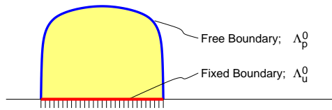
Fig. 4. Reference Boundary Value Problem (RBVP) Definition : The RBVP associated with a model attached to a flat rigid support is shown with boundary regions having displacement (“fixed”, \Lambda_u^0 ) or traction (“free”, \Lambda_p^0 ) nodal constraints indicated. A typical simulation would then impose contacts on the free boundary via displacement constraints with the capacitance matrix algorithm.
