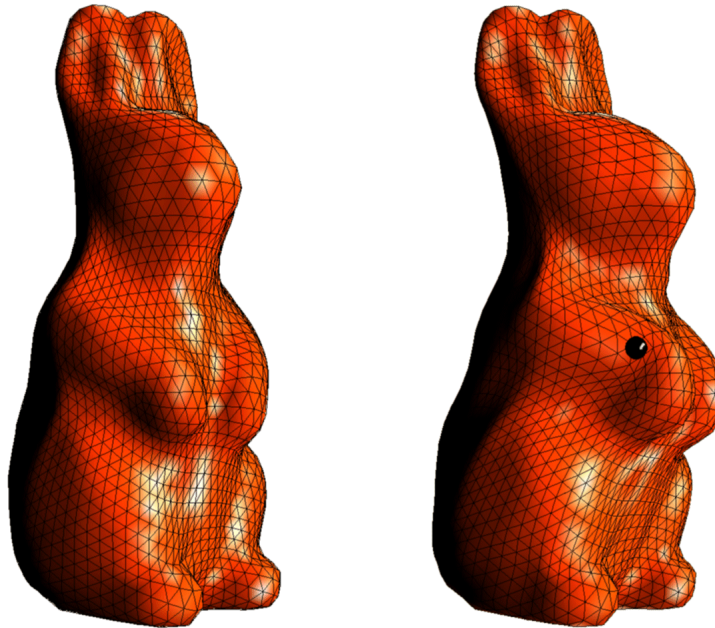
Fig. 1. Preview of Results for a Complex Elastic Model: An elastic rabbit model with 2562 vertices, 5120 faces and 5 levels of subdivision connectivity ( L = 4 ), capable of being rendered at 30 FPS with 1 kHz force feedback on a PC in our Java-based haptic simulation. The associated dense square Green's function (GF) submatrix contained 41 million floats (166 MB) but was compressed down to 655 thousand floats (2.6 MB) in this animation ( \epsilon = .2 ). The depicted deformation resulted from force interactions defined at a constraint resolution that was two levels coarser ( L=2 ) than the visible mesh; for these coarse level constraints, the GF matrix block may be further compressed by a factor of approximately 16 = 4^2 . Even further compression is possible with file formats for storage and transmission of models. (Reparameterized rabbit model generated from mesh courtesy of [Cyberware].)
