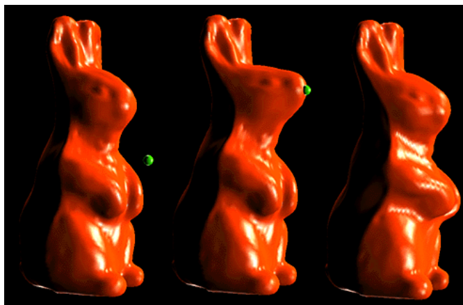
Fig. 12. Elastically Deformed Displaced Subdivision Surfaces : Displaced subdivision surfaces provide a natural extension to an hierarchy of elastic spatial scales. In this example, a level 2 elastic rabbit model is rendered on level 5 using displacement mapping (computed in software). In addition to providing exact displacement constraints on detailed (or just subdivided) surfaces, hierarchical GFs allow greater elastic content to be depicted than simple displacement mapping of coarse geometry. In either case, such approaches can effectively transfer the runtime simulation burden almost entirely to graphical rendering.
