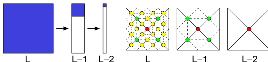
Fig. 11. Hierarchical Capacitance Matrices : (Left) As in Figure 9, the matrix view of hierarchical GF indicates an approximately four-fold reduction in columns at each coarser constraint resolution. As a result, the number of possible capacitance matrix elements are reduced accordingly, as represented by the blue matrix blocks. (Right) An illustration of the corresponding spatial hierarchy for the support of a coarse level (extraordinary) ‘linear hat’ scaling function. Circles indicate the vertex nodes (and basis functions) required to represent the coarse level scaling function at each level.
