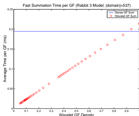
Fig. 17. Fast summation cost per GF summed : Comparison of wavelet GF fast summation timings (in milliseconds) of a rabbit model ( L = 3 , 537 vertex domain) with dense GF matrix multiplication (horizontal line, time=0.19ms/GF) for full matrix multiplication. The linear dependence on nonzero GF matrix elements confirms the cost analysis of §5.5 (equation 50, p. 19): fast summation costs are directly proportional to the number of nonzero wavelet GF elements. Timings are for the lifted Linear wavelets, for which the inverse FWT requires 0.38 ms.
