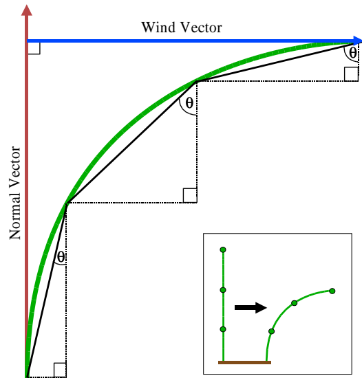
Figure 6: The Length-Preserving Function to Bend a Blade of Grass.
