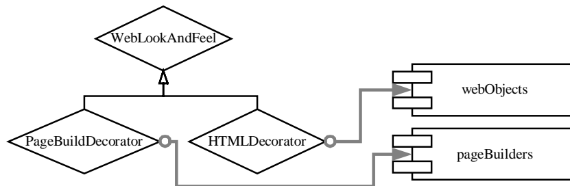
Figure 7 Modularizing Look-and-Feel
