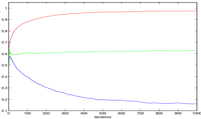
Figure 2: Sequence of parameter estimates for RML \theta_n = (\sigma_n, \phi_n, \beta_n) for N = 1000 . From top to bottom: \phi_n , \beta_n and \sigma_n .
