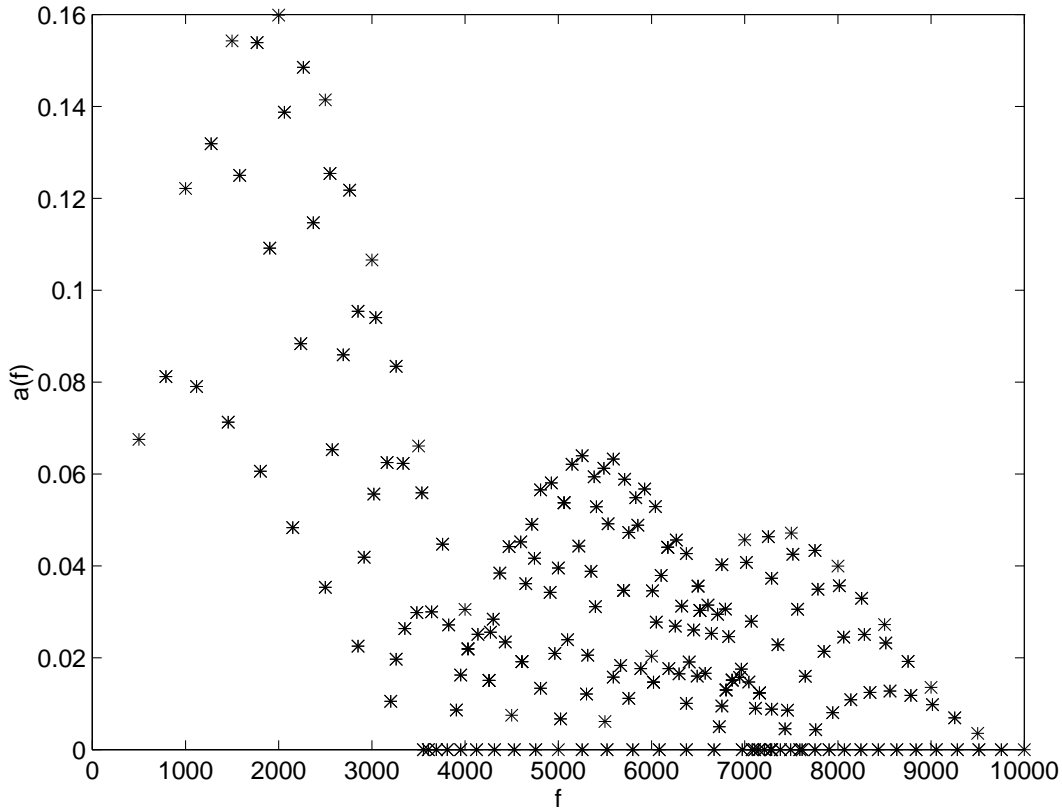
Figure 2: Square membrane struck at (0.1, 0.1)
