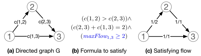
Figure 2: (a) Example symbolic graph, with variable capacities c(u, v) on each edge. includes the capacity assigned to each edge, as well as the flow along that edge. (b) A formula constraining the graph. (c) A solution, assigning a flow and a capacity ( f/c ) to each edge.
