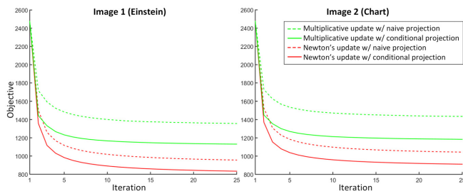
Fig. 11. Convergence for two factorization methods (rank 1 factorization on a 1,751 by 1,751 pixel target image) with and without projection (Eq. 11). The two images tested are same as in Fig. 5.
