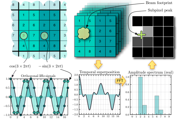
Figure 3: Left: Sample 4x4 tile. In this case, f_{\max} = 8\text{Hz} . The phase is 0 in the left half of the tile and \pi/2 in the right. Right: Temporal superposition of signals under the beam footprint.
