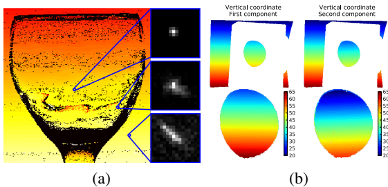
Figure 5: (a) Examples of spread-out, bimodal and point-like point spread functions. The color gradient indicates the vertical component of the detected background pixels' coordinates. (b) Multipath correspondences. A beamsplitter inside the occluder reflects some light onto a mirror that directs it to another point on the illuminant. The bottom row of images show a closeup of the central region (the beamsplitter) on a different color scale.
