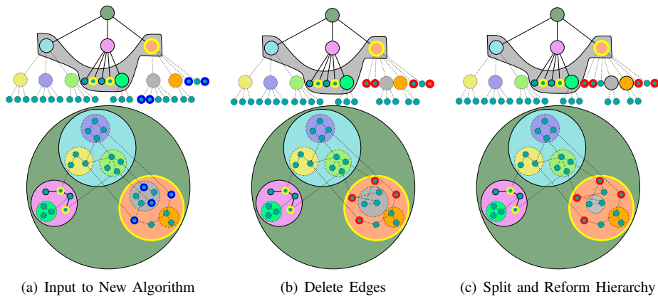
Fig. 6. New steps for hierarchy modification. (a) The input is the proximal set as in the previous version of the algorithm. (b) Proximal components are tugged out and edges are deleted. The grey metanode is now disconnected. (c) Grey metanode is split in two to preserve connectivity conservation. Edge deletions followed by splits are propagated up the hierarchy until the cut metanodes are reached.
