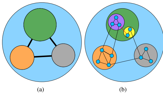
Fig. 3. The importance of edge and connectivity conservation in understanding paths when using a graph hierarchy. A more complete version is presented in GrouseFlocks [6]. (a) Top level of graph hierarchy consisting of three metanodes with a cycle. (b) Underlying graph and graph hierarchy. If the red edge does not exist, there appears to be a cycle at the top level of the hierarchy when no such cycle exists in the underlying graph. If edge conservation is not respected, we are unsure if metaedges on the cut really exist. If connectivity conservation is not respected, as in this example, we are unsure if paths in the underlying graph actually exist.
