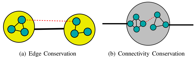
Fig. 2. Edge conservation and connectivity conservation are required to preserve paths in hierarchy cuts. (a) Edge conservation ensures that edges exist between metanodes of a hierarchy cut if and only if there exists one or more edges between descendants of the metanodes. (b) Connectivity conservation ensures that paths exist through metanodes. If the red dashed edge did not exist, there would not be a path from the bold metaedge on the left through to the bold metaedge on the right.
