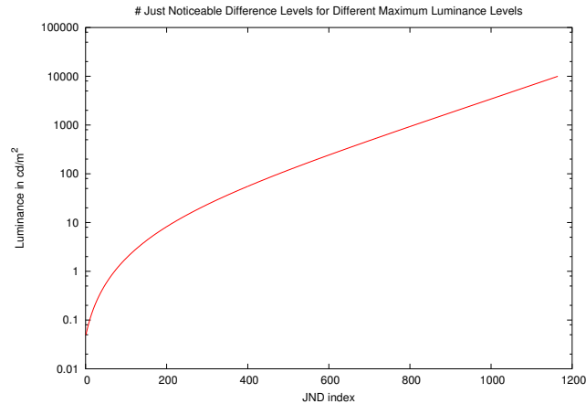
Figure 3: The number of just noticeable difference (JND) steps for different maximum intensities according to the model by Barten [1992,1993].
