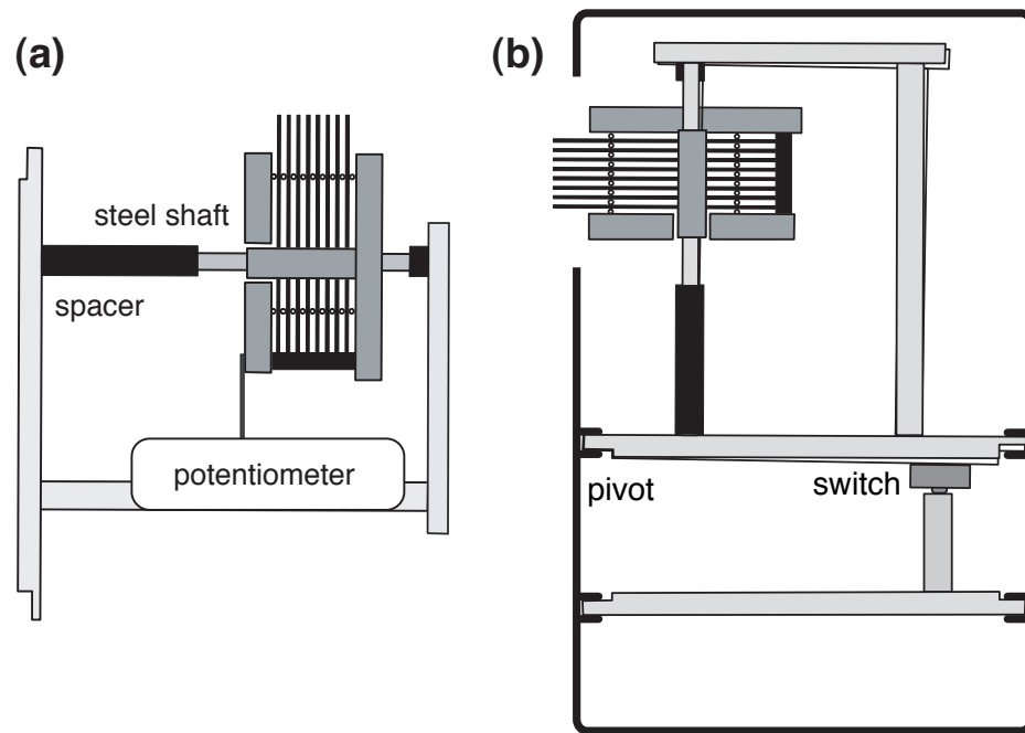
Figure 4.4: Location of input sensors. (a) Resistive position sensor. (b) Push-to-select sensor. Diagrams by Jerome Pasquero.
