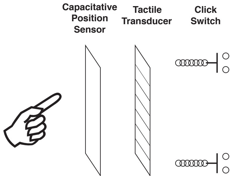
Figure 3.3: Schematic diagram of a concept bidirectional haptic device for 1-D linear input and tactile output. A flexible sensor for determining the position of the user's finger is layered on top of a deformation-producing tactile output transducer, and mounted on a movable apparatus so that the force of the user's finger pressing into the device can be detected for actions such as selection. (Components not drawn to scale)
