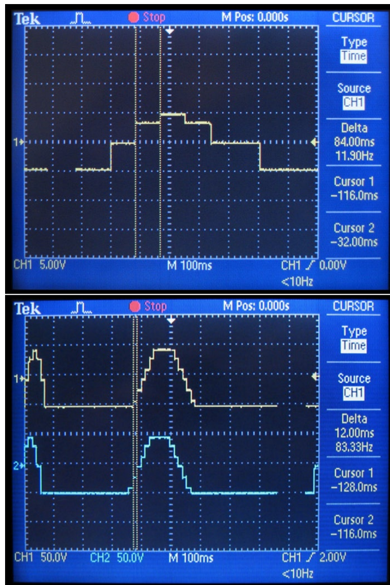
Figure 4.5: Measured outputs under conditions of load (running the browser application). Above , prior to optimization. Below , after optimization, showing two adjacent output channels at once.
