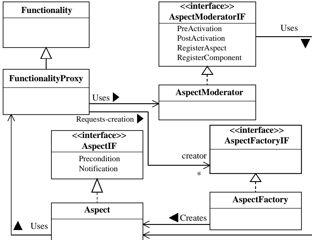
Figure 2. The architecture of the aspect moderator framework.
