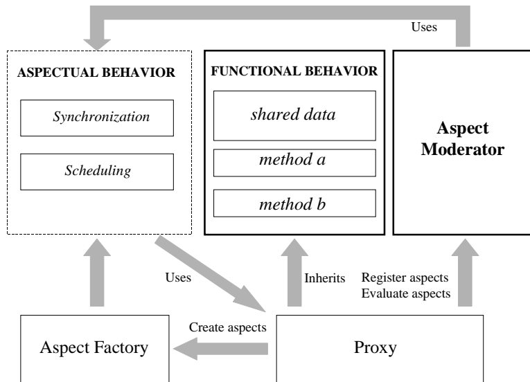
Figure 1. The aspect moderator framework as a cluster of cooperating objects.
