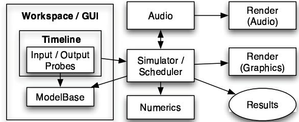
Figure 1: Association diagram of the main components of ArtiSynth. The arrows indicate the general control relationships between the components.
