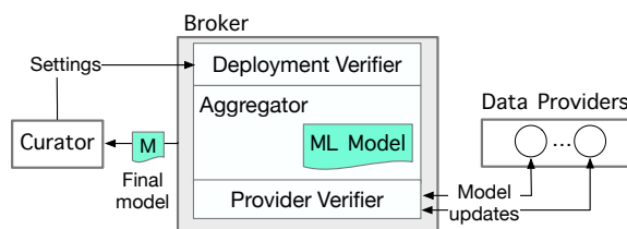
Figure 2: Overview of brokered learning.
