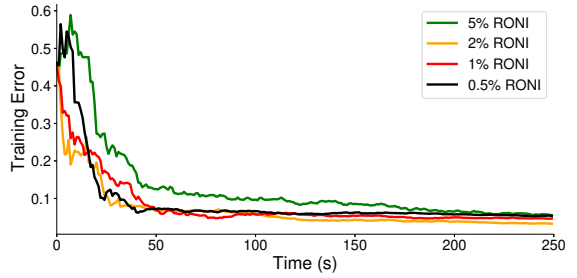
Figure 7: Training error over time, when attacked by 50% poisoners. RONI threshold is varied 0.5% – 5%.
